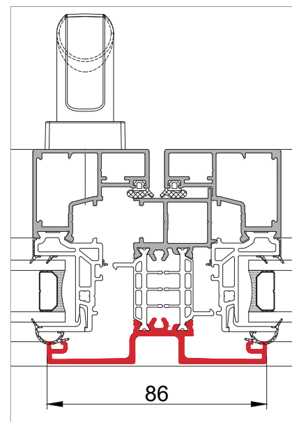
Battue standard
