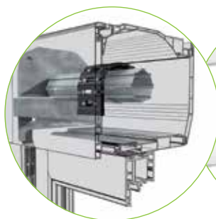
SYSTÈME ANTI-RELEVAGE
